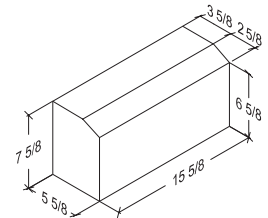
6 x 8 x 16 - Chamfer A 5 3/8" x 7 3/8" x 15 5/8"
