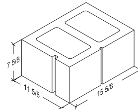
12-8-16 1-Score 11 5/8" x 7 3/8" x 15 5/8"
