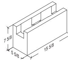
6-8-16 Bond Beam 5 5/8" x 7 3/8" x 15 5/8"
