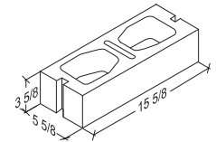
6-4-16 Half High Partition 5 5/8" x 3 5/8" x 15 5/8"
