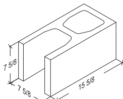
8-8-16 Conduit 7 5/8" x 7 5/8" x 15 5/8"
