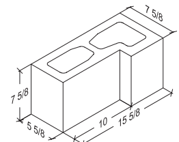
6 Inch L-Corner 7 5/8" x 7 3/8" x 15 5/8"
