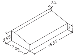
8 x 4 x 16 Slope Sill 9 7/8" x 3 3/8" x 15 5/8"
