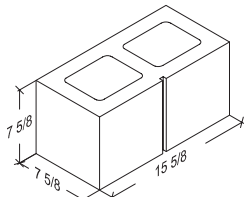
8-8-16 1-Score 7 5/8" x 7 5/8" x 15 5/8"
