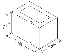
12-8-8 Half 11 5/8" x 7 3/8" x 7 3/8"
