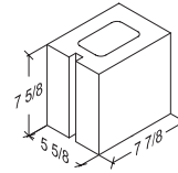
6-8-8 Half 5 5/8" x 7 3/8" x 7 7/8"
