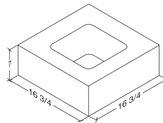
17 x 7 x 17 Chimney Block 16 3/4" x 7" x 16 3/4"
