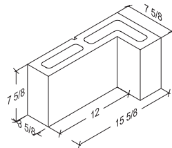
4 Inch L-Corner 7 5/8" x 7 3/8" x 15 5/8"
