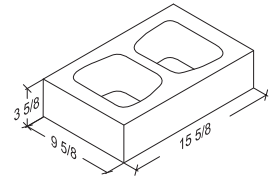
10-4-16 Half High 9 5/8" x 7 5/8" x 15 5/8"
