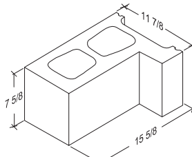
12-8-16 L-Corner 11 5/8" x 7 3/8" x 15 5/8"
