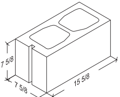
8-8-16 Square Corner 7 5/8" x 7 5/8" x 15 5/8"
