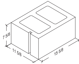
12-8-16 Square Corner 11 5/8" x 7 3/8" x 15 5/8"
