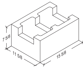
12-8-16 Bond Beam 11 5/8" x 7 3/8" x 15 5/8"
