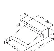
10 x 4 x 8 Square Sill 9 7/8" x 3 3/8" x 7 3/8"
