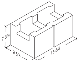
10-8-16 1-Score Bond Beam 9 5/8" x 7 5/8" x 15 5/8"
