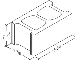
10-8-16 Standard 9 5/8" x 7 5/8" x 15 5/8"
