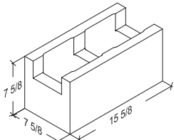
8-8-16 Bond Beam 7 5/8" x 7 5/8" x 15 5/8"
