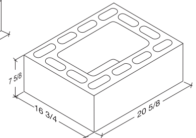
17 x 8 x 21 Chimney Block 16 3/4" x 7 3/8" x 20 5/8"
