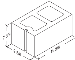
10-8-16 Square Corner 9 5/8" x 7 5/8" x 15 5/8"
