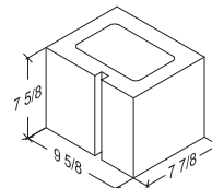
10-8-8 Half 9 5/8" x 7 5/8" x 15 5/8"
