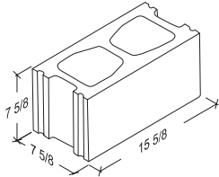
8-8-16 Standard 7 5/8" x 7 5/8" x 15 5/8"
