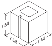
8-8-8 Half 7 5/8" x 7 5/8" x 7 7/8"
