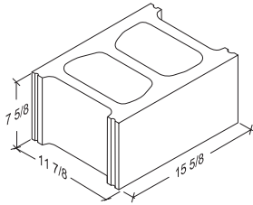
12-8-16 Standard 11 7/8" x 7 3/8" x 15 5/8"
