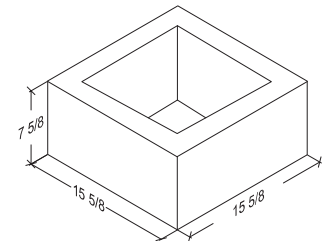
16 x 8 x 16 Chimney Block 15 5/8" x 7 3/8" x 15 5/8"
