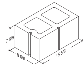
10-8-16 1-Score 9 5/8" x 7 5/8" x 15 5/8"
