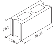
6-8-16 Standard 5 5/8" x 7 3/8" x 15 5/8"
