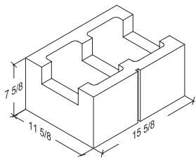
12-8-16 1-Score Bond Beam 11 5/8" x 7 3/8" x 15 5/8"
