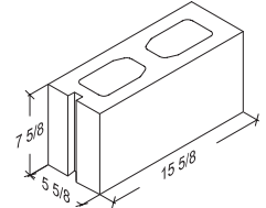
6-8-16 Square Corner 5 5/8" x 7 3/8" x 15 5/8"
