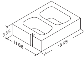
12-4-16 Half High 11 5/8" x 3 5/8" x 15 5/8"
