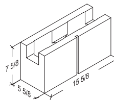
6-8-16 1-Score Bond Beam 5 5/8" x 7 3/8" x 15 5/8"
