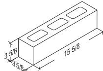
4-4-16 Half High Partition 3 5/8" x 3 5/8" x 15 5/8"
