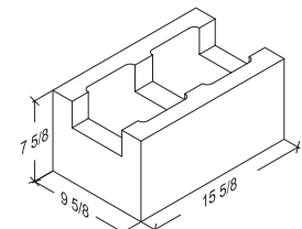
10-8-16 Bond Beam 9 5/8" x 7 5/8" x 15 5/8"
