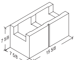
8-8-16 1-Score Bond Beam 7 5/8" x 7 5/8" x 15 5/8"
