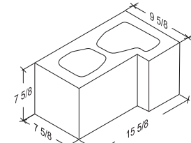
10-8-16 L-Corner 9 5/8" x 7 5/8" x 15 5/8"
